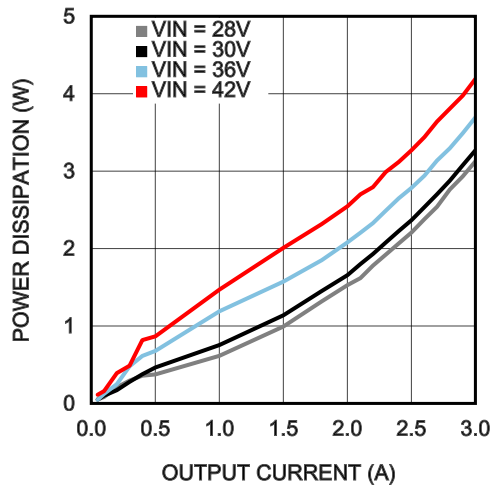
Power Dissipation V_{OUT} = 24V T_{AMB} = 25^{\circ}C
