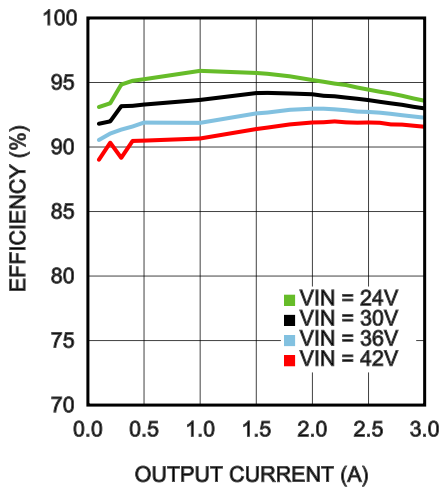
Efficiency V_{OUT} = 18V T_{AMB} = 85^{\circ}C
