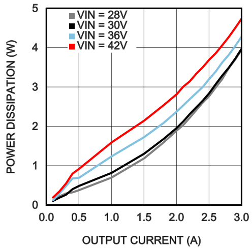
Power Dissipation V_{OUT} = 24V T_{AMB} = 85^{\circ}C
