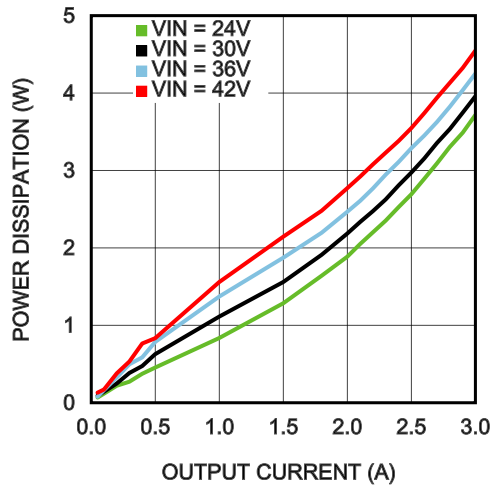
Power Dissipation V_{OUT} = 15V T_{AMB} = 85^{\circ}C
